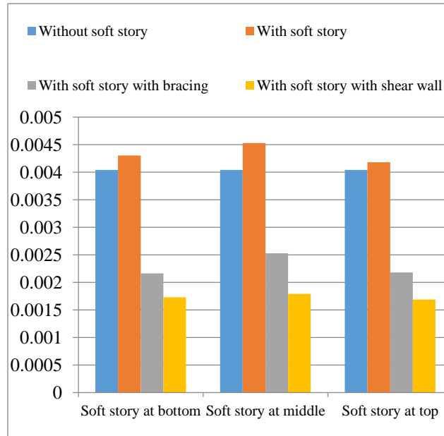
Chart -5: Maximum values of Story Drift in Y direction
