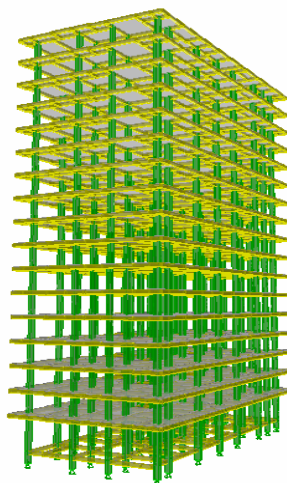
Fig -3: Elevation view of building with soft story at bottom in ETABS
