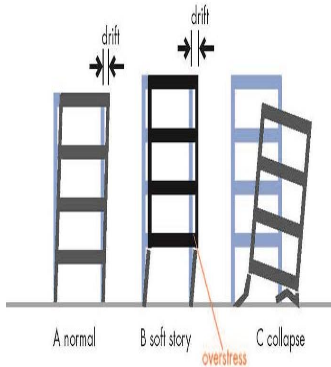
Fig -1: Soft story failure
