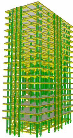
Fig -5: Elevation view of building with soft story at bottom with Bracing in ETABS
