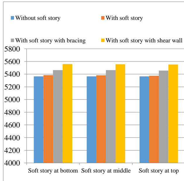
Chart-1: Maximum values of Story Shear in X direction
