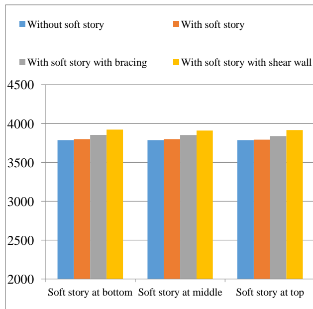
Chart-2: Maximum values of Story Shear in X direction
