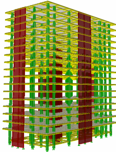
Fig -4: Elevation view of building with soft story at bottom with shear wall in ETABS
